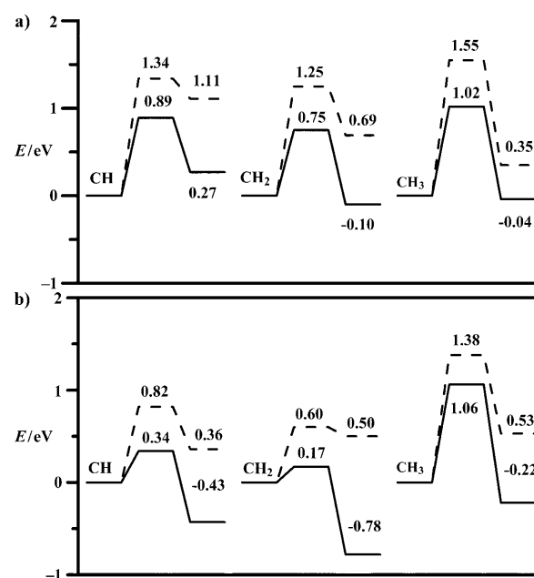
Figure 1. Calculated barriers and reaction energies for CO (dashed line) and HCO (solid line) insertion into \text{CH}_x ( x=1-3 ) on a) Rh(111) and b) Co(0001) surfaces.
