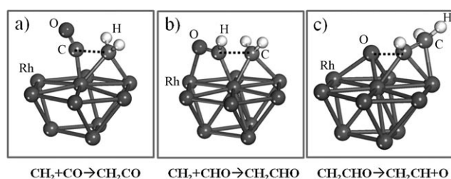
Figure 3. Structures of the optimized transition state for a) CO and b) HCO insertion into \text{CH}_2 and c) C=O bond scission of \text{CH}_2\text{CHO} on a Rh(111) surface.
